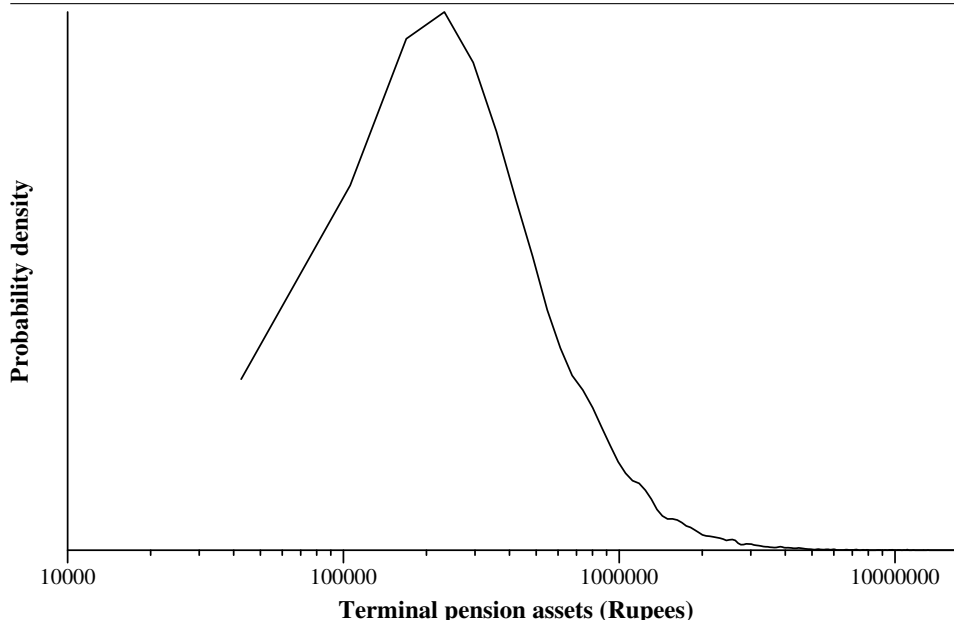
Figure 1 Distribution of V_T : One example ( W_0 = 50 and \lambda = 1 )
